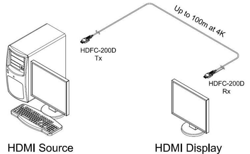
Figure 1 – General connection diagram of HDFC-200D
