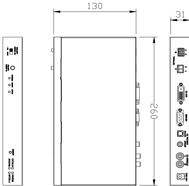
Transmitter
