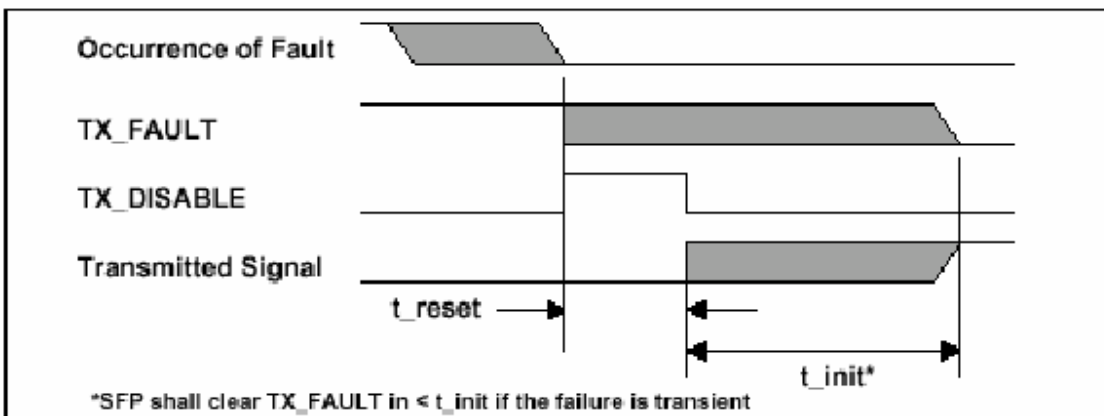
Figure 8. Successful recovery from transient safety fault condition
