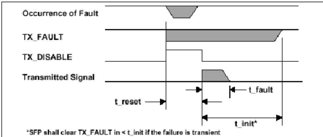
Figure 9. Unsuccessful recovery from safety fault condition
