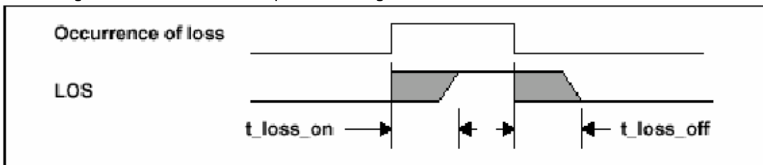
Figure 10. Timing of LOS detection
