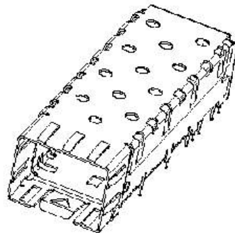
Figure. 12 Drawing of Cage for SFP Transceivers
