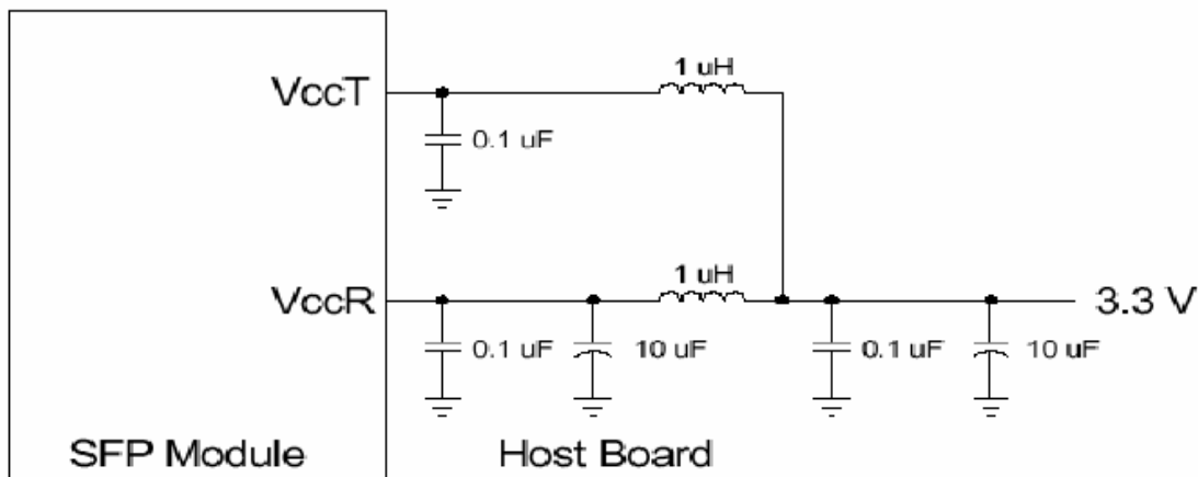
Figure 1. Recommended Host Board Supply Filtering Network
