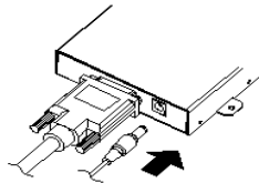
Figure 5 – Connection of AC/DC power adaptor
