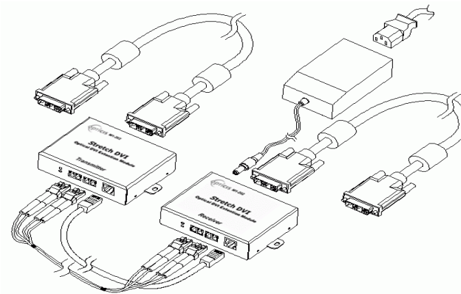
Figure 1 – Overall Optical DVI Module
