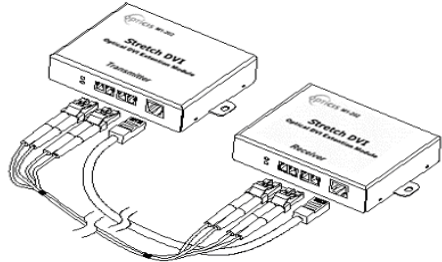
Figure 4 – Connection of 2 duplex LC fiber cables
