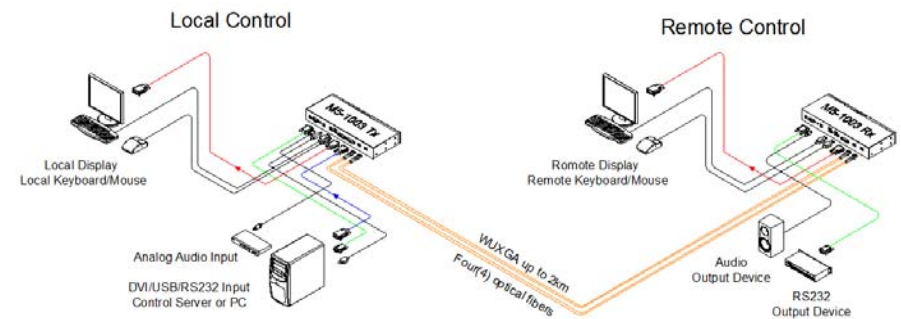
Figure 1 – Overall connection of M5-1003 Optical KVM Extender
