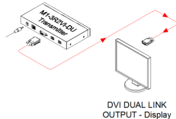
Figure 6 – Connection for Self-EDID programming
