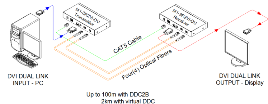
Figure 1 – Overall Optical dual link DVI Module
